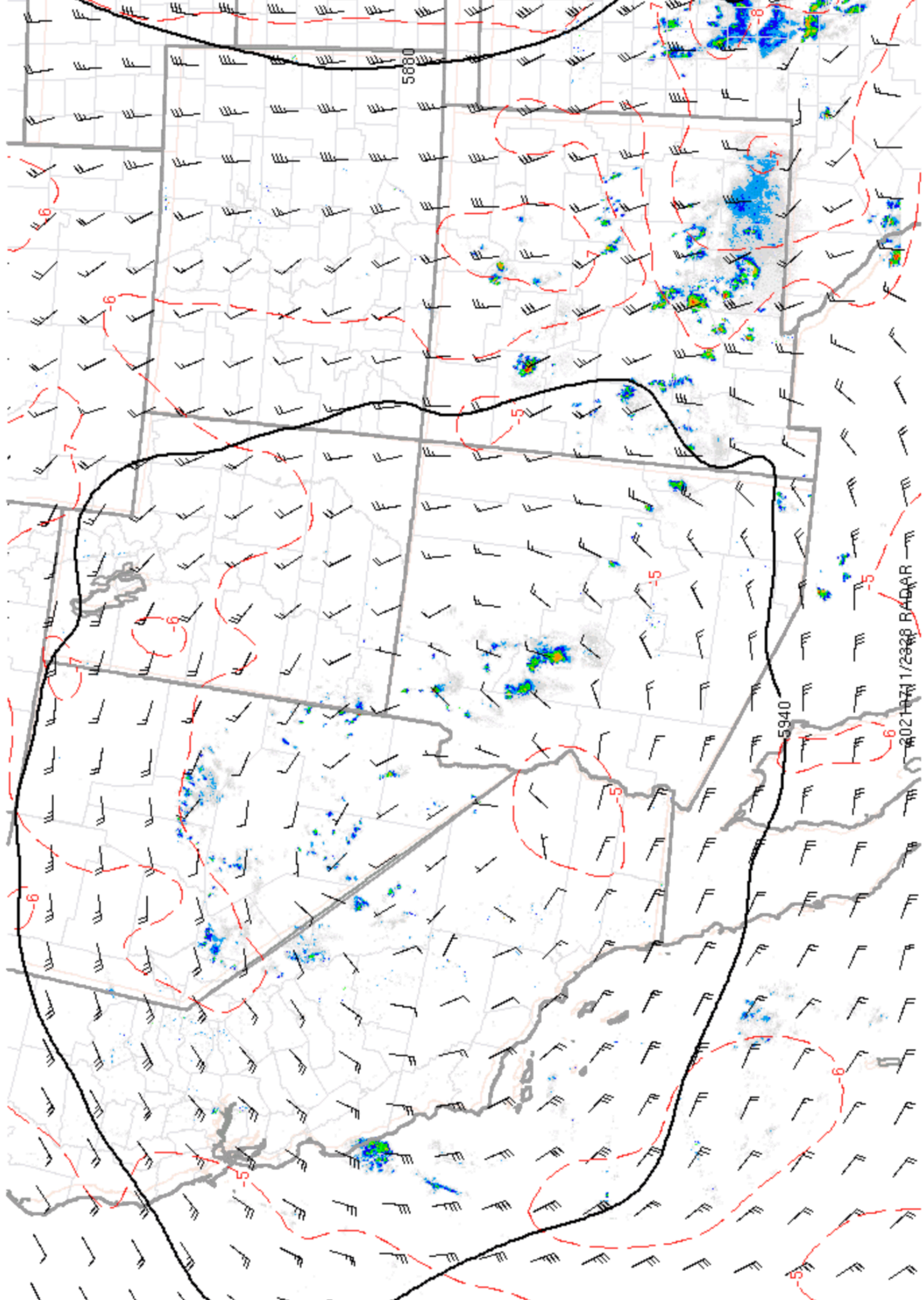
210711/2300V001 500mb height (m MSL, black), temp (C, red), and wind (kt, hatched >= 40 kt)
