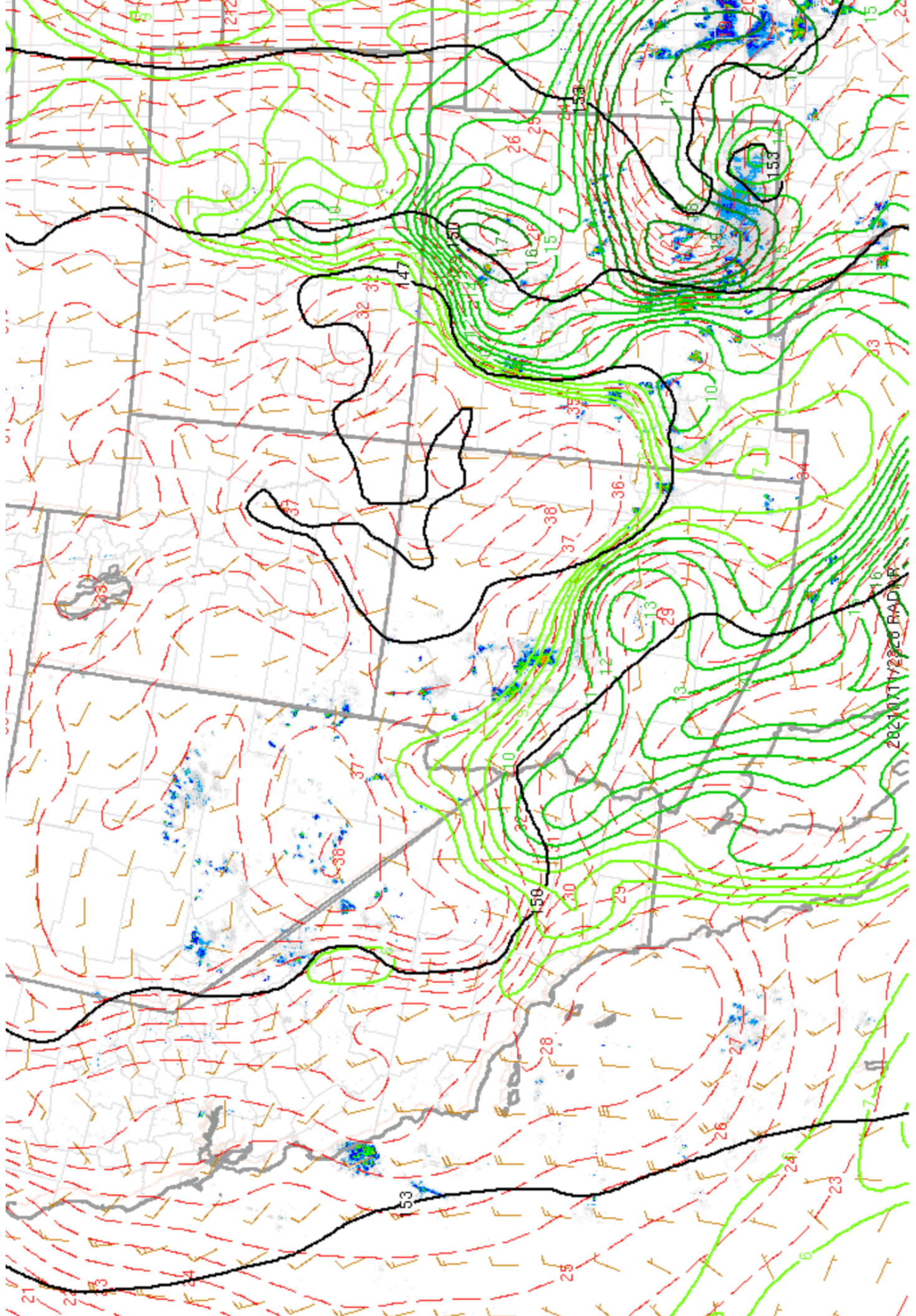
210711/2300V001 850mb height (m MSL, black), temp (C, red), dewpoint (C, green), and wind (kt)
