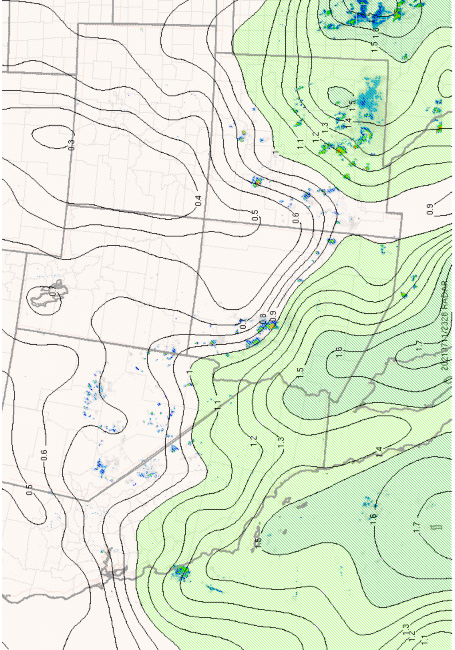
210711/2300 precipitable water (in) lowest 400 mb
