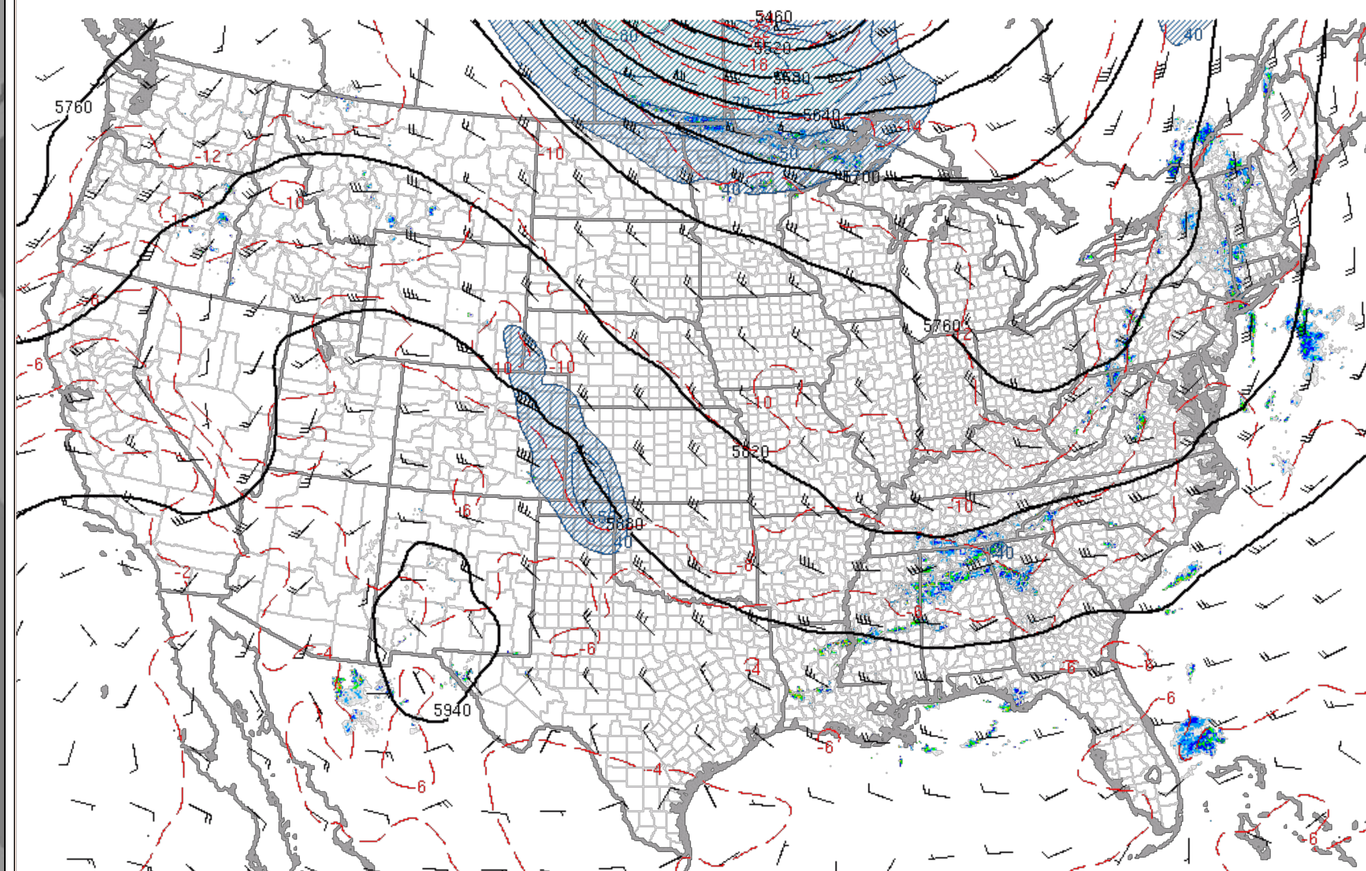
230710/0200V001 500mb height (m MSL, black), temp (C, red), and wind (kt, hatched >= 40 kt)
