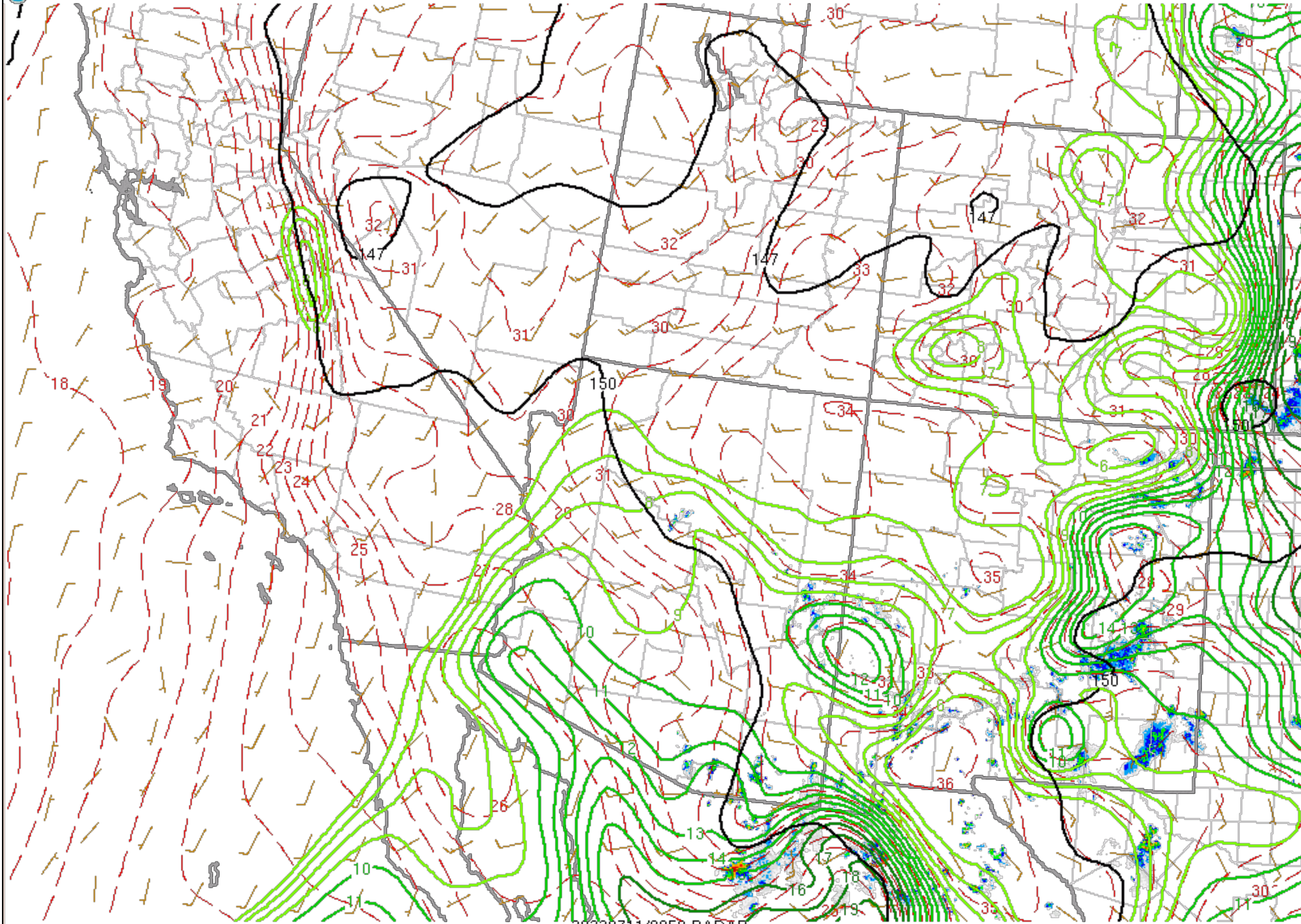
230711/0000V001 850mb height (m MSL, black), temp (C, red), dewpoint (C, green), and wind (kt)
